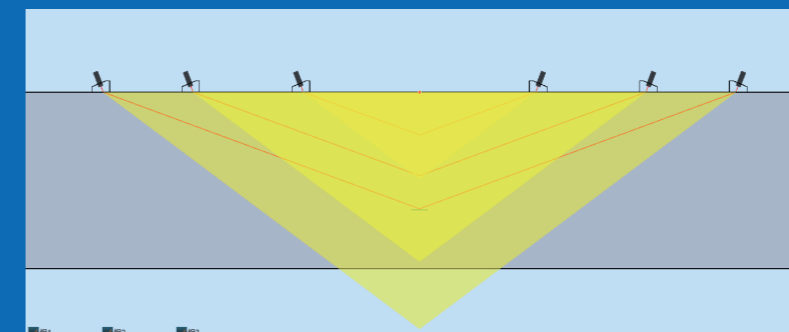
Multi-group TOFD coverage simulation
