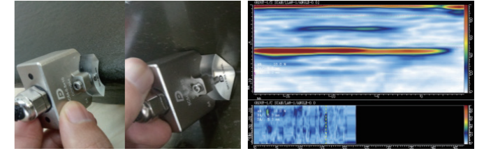
Aircraft CFRP Composite R Corner Inspection(Concave Probe)
