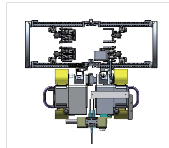
The illustrated holding frame can hold a 32-element or 64-element phased array probe.
