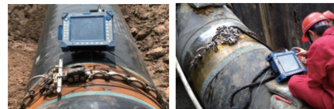
Circumferential Weld Inspection of Oil and Gas Pipelines
