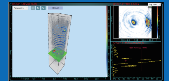
Bolt 3D TFM inspection
