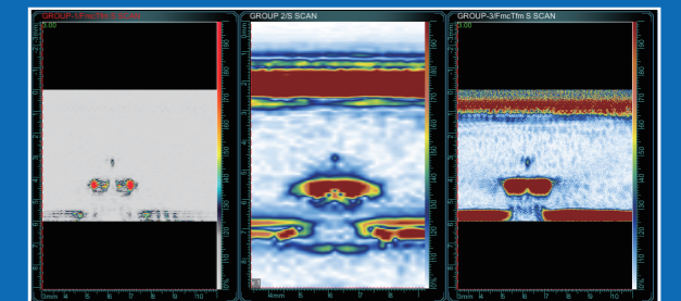
Copper, φ0.1mm flat bottom hole, FMC-PCI(left), PA(center), FMC-TFM(right)
