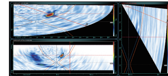
Detection of CRA weld test block
