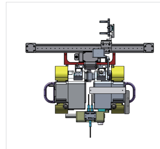
The illustrated probe holding arm can hold a 128-element phased array probe.
