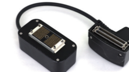
T1(Male)-H1(Female) H1(Probe)-T1(Instrument)
