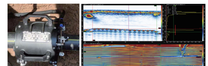
Inspection of PE electrofusion joint
