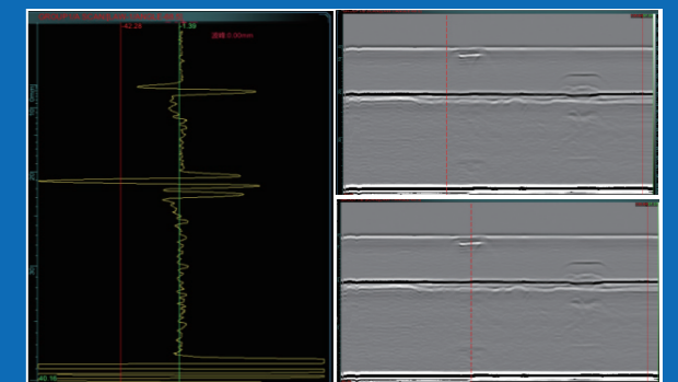
TOFD weld detection
