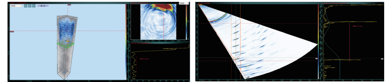
Bolt 3D TFM imaging
