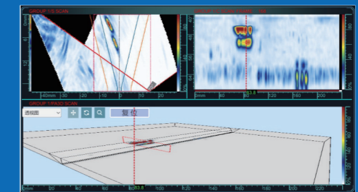
PA-3D Scanning
