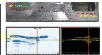
FSW friction stir welding inspection
